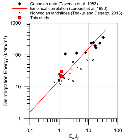
Figure 10 Disintegration energy of Norwegian and Canadian clays (from Thakur et al. 2015)
